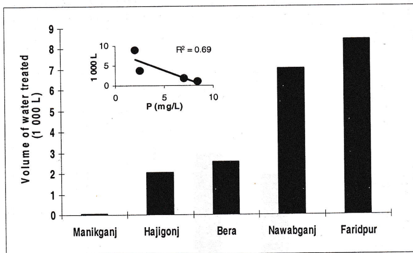
Figure 4. Bar chart showing the regional performance of the Ferric coated activated alumina (FAA) filters along with the linear graph showing the correlation between groundwater total inorganic phosphate (reported as elemental P) and filter performance. The filled in bars in the chart represent filters that had attained breakthrough during the duration of the study where as the empty bars represent filters that did not attain breakthrough during the duration of the study.
