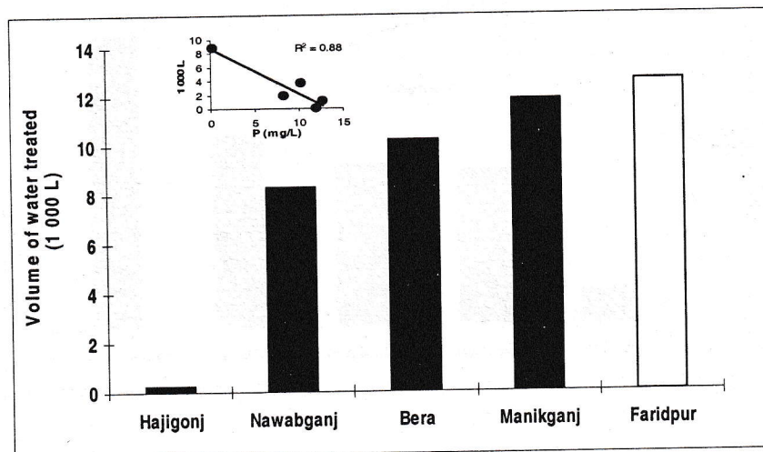
Figure 6. Bar chart showing the regional performance of the Zero valent iron based (ZF) filters along with the linear graph showing the correlation between groundwater total inorganic phosphate (reported as elemental P) and filter performance. The filled in bars in the chart represent filters that had attained breakthrough during the duration of the study where as the empty bars represent filters that did not attain breakthrough during the duration of the study.
