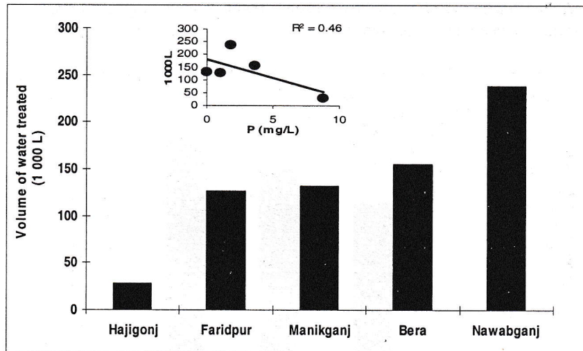
Figure 5. Bar chart showing the regional performance of the Granular ferric hydroxide based (GFH) filters along with the linear graph showing the correlation between groundwater total inorganic phosphate (reported as elemental P) and filter performance. The filled in bars in the chart represent filters that had attained breakthrough during the duration of the study.
