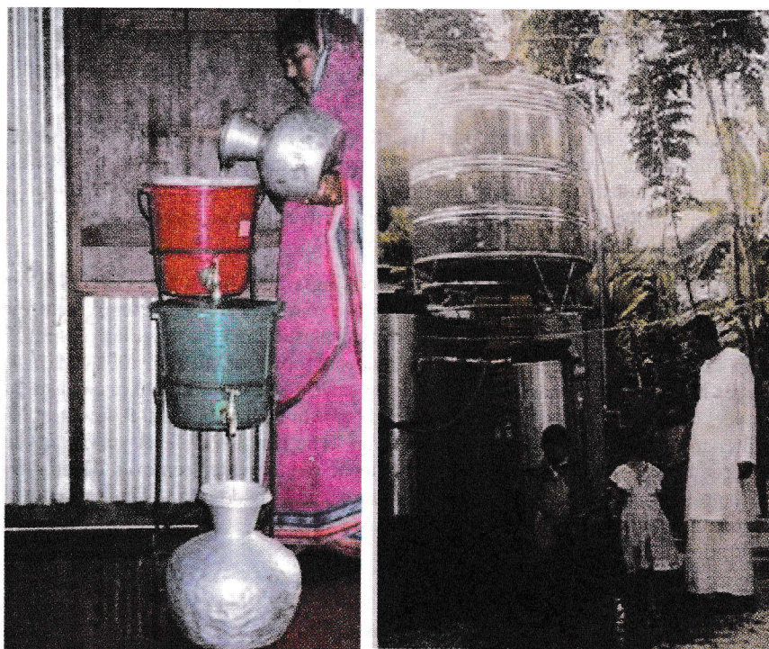
Figure 1. Pictures of household and community level arsenic removal filters being used in rural Bangladesh.
